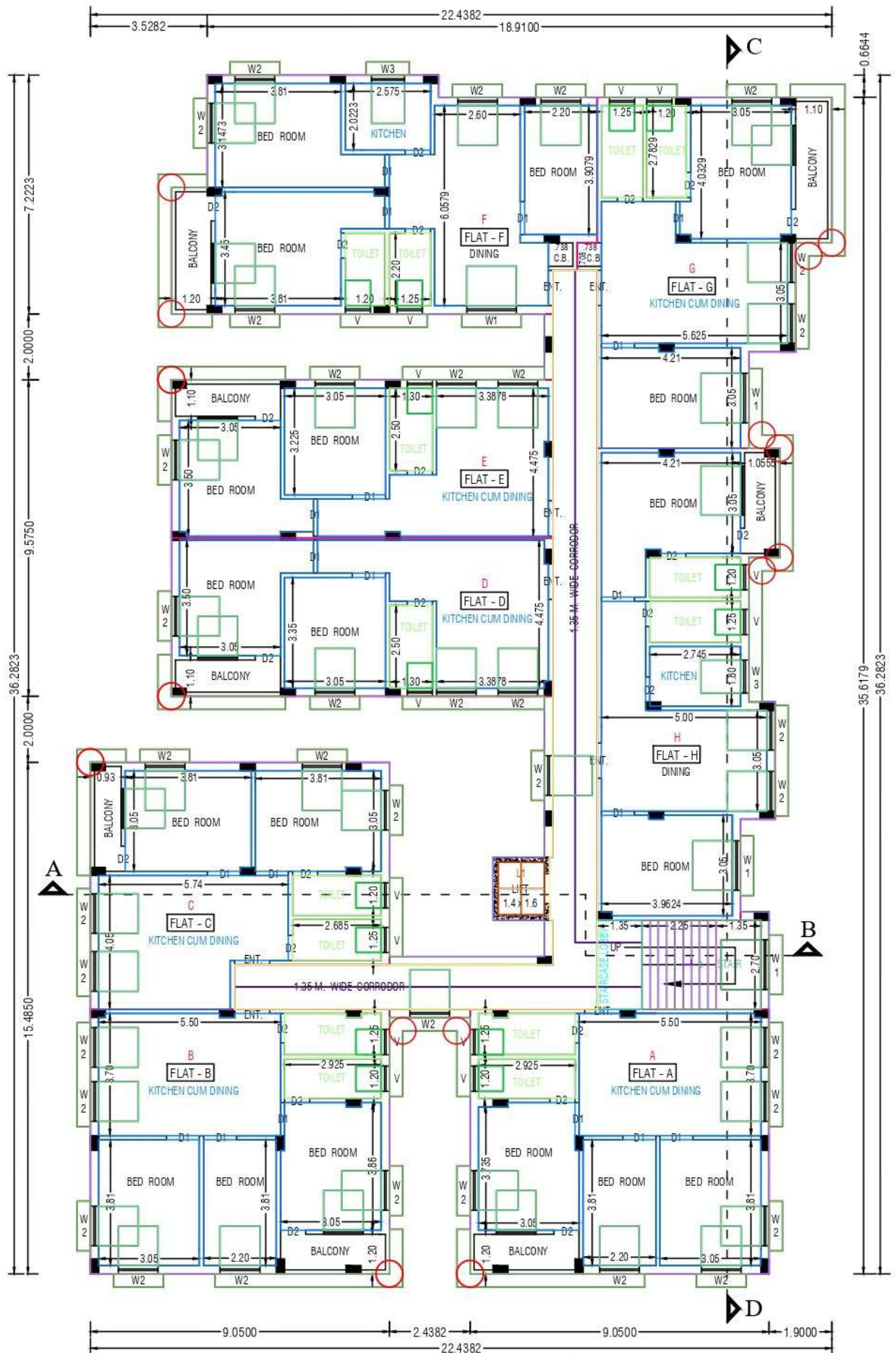
FLOOR01,FLOOR02,FLOOR03-TYPICAL (PROPOSED FIRST, SECOND & THIRD FLOOR PLAN)
